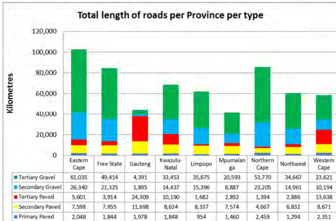
Figure 50: Total length of road type per province
