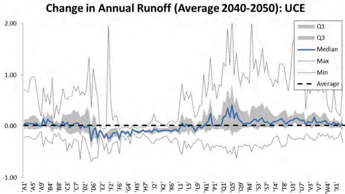
Figure 15: Range of potential impacts of climate change on the average annual catchment runoff for all secondary catchments for the period 2040 to 2050 due to the UCE scenario relative to the base scenario
