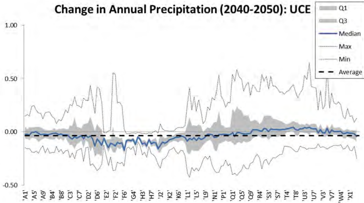
Figure 6: Range of potential impacts on the change in the average annual precipitation by 2050 in each secondary catchment of South Africa under the UCE climate scenario
