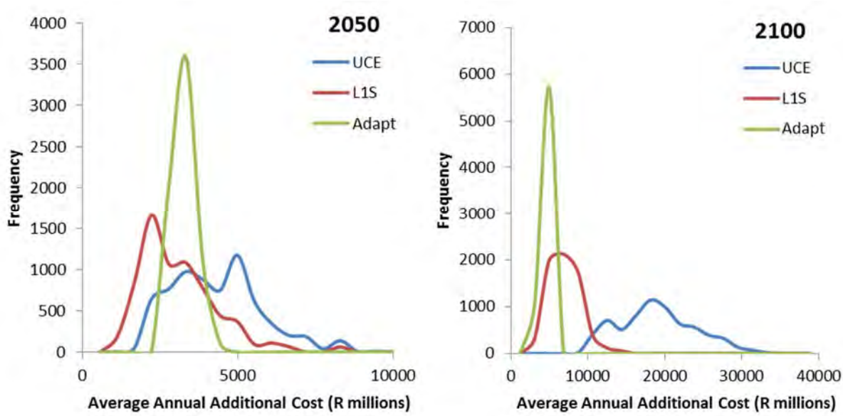
Figure 52: Range of potential impacts of future climate change scenarios on the decadal average annual additional costs for roads infrastructure in South Africa by 2050 and 2100 under the 'adapt' and 'no adapt' management scenarios
