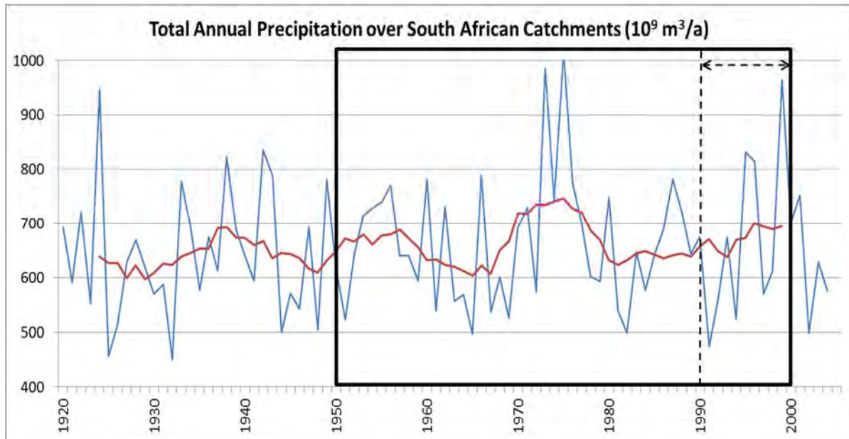
Figure 22: Total annual precipitation over South African catchments (10 9 m 3 /a) showing the period 1950 to 2000 used as the base scenario for simulation of the climate change impacts from 2000 to 2050. Also indicated is the last ten year period used to determine the potential impacts by mid-century.
