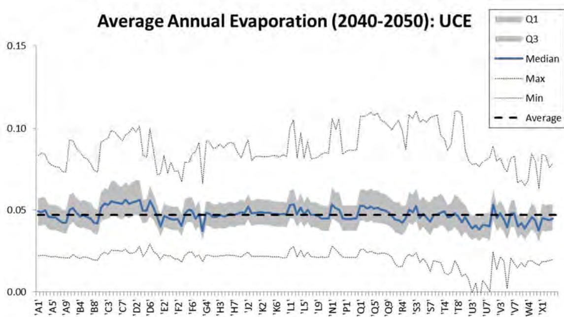
Figure 1: Range of potential impacts on the change in the average annual evaporation by 2050 in each secondary catchment of South Africa under the UCE climate scenario
